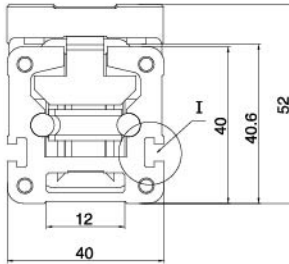
I 用于模组固定块固定和安装外置开关座 intallation of cable duct and outside switch sockt
